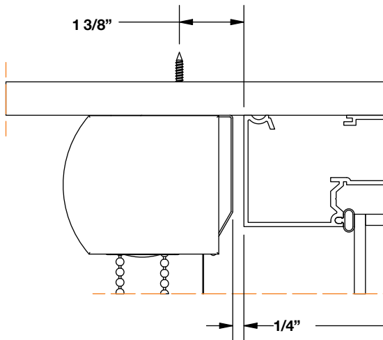
Ceiling Mount
