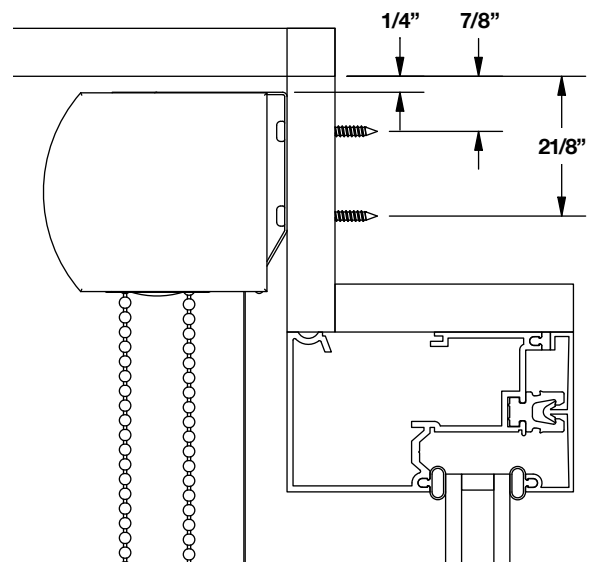
Wall Mount
