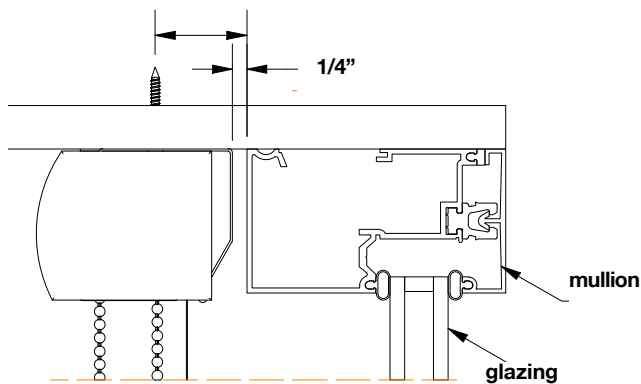
Ceiling Mount
