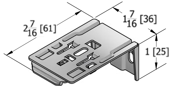
ISOMETRIC VIEW (Bracket Size)
