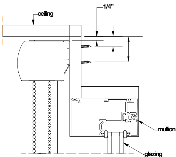
Wall Mount
