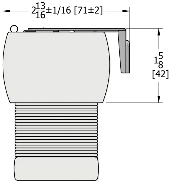
SIDE PROFILE
