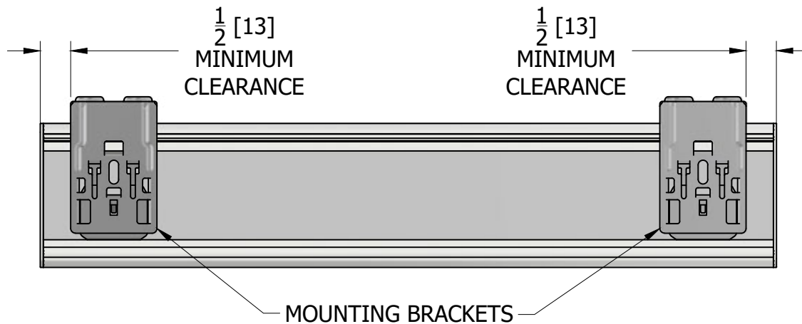
TOP VIEW (Bracket Spacing)
